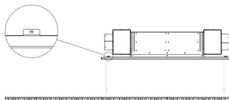
Safety Cable Mounting Point
