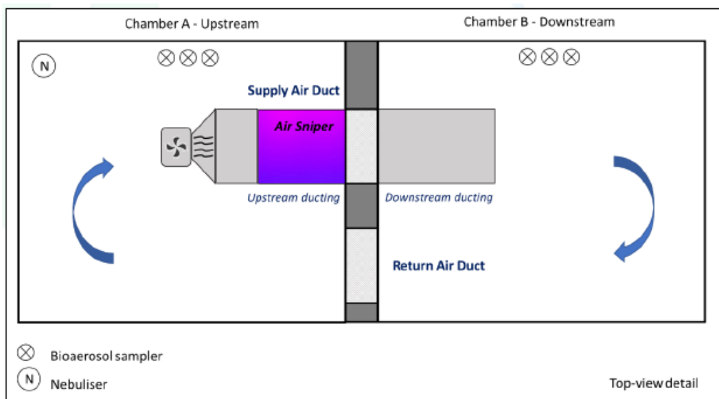
Figure 3.1. Multi-chamber Test Setup for MS2 Testing
